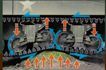
Free spinning wheels & real vertical volute spring suspension design.
