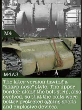
The later version having a "sharp-nose" style. The upper border, along the bolt strip, also evolved, so that the bolts were better protected against shells and explosive devices.
