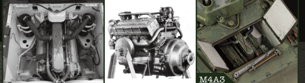
The GAA V8 engine that powered the M4A3 Sherman tank and several other vehicles based on the Sherman chassis.
