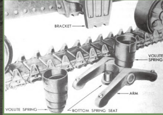
Bogie assembly, Vertical volute spring, with the "offset roller" and skid. The most common type that can be found on Sherman tanks.
