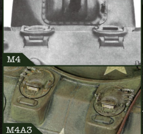
The drivers' hoods were redesigned to eliminate them. The hoods were elongated in the front, where an additional periscope was provided.
