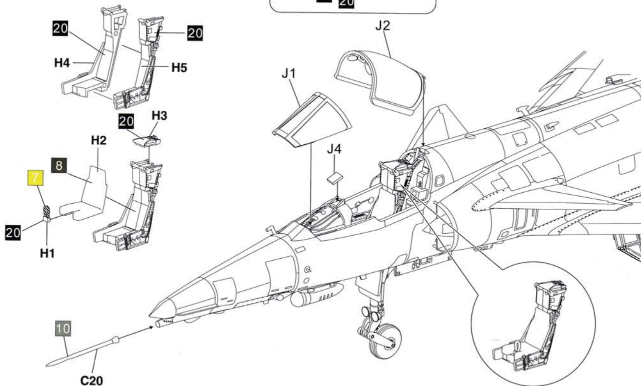
Mk. IN10LH ejection seat
