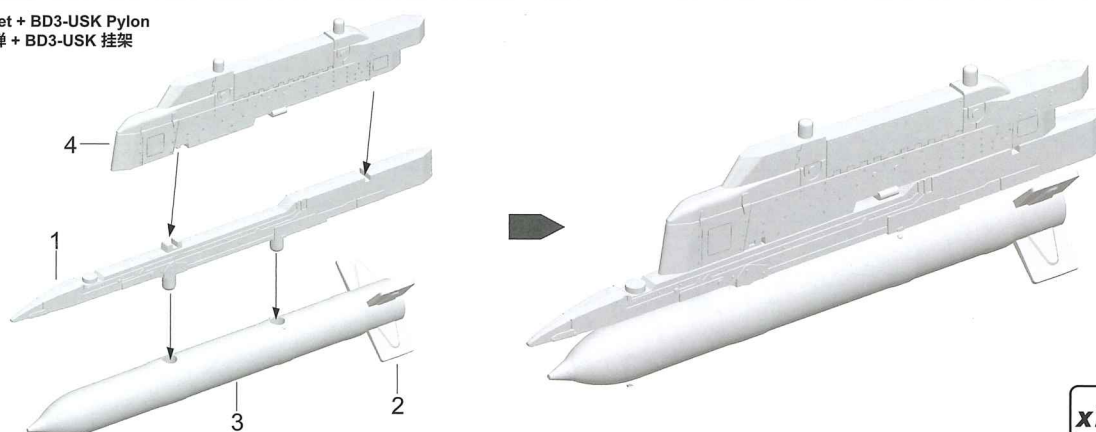
B-8M1 Launcher + BD3-USK Pylon B-8M1 火箭巢 + BD3-USK 挂架
