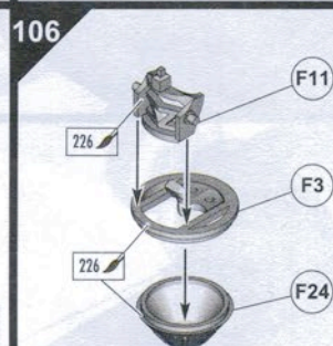
Rear Turret Assembly
