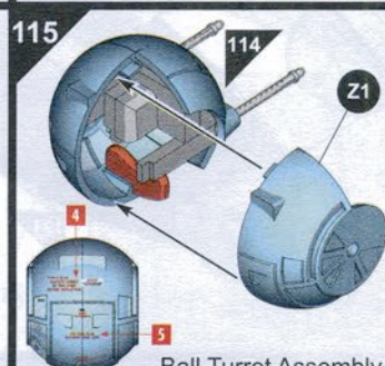
Ball Turret Assembly
