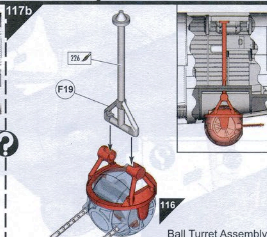
Ball Turret Assembly
