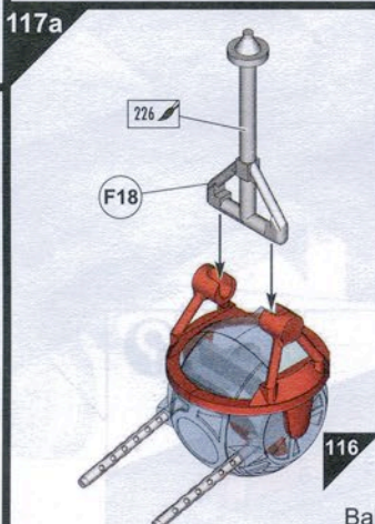
Ball Turret Assembly
