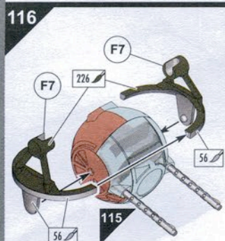
Ball Turret Assembly
