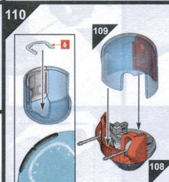
Nose Turret Assembly
