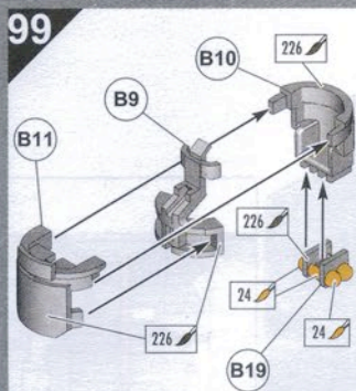
Top Turret Assembly
