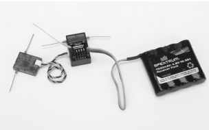
Shown using a separate receiver pack. (Battery can be plugged into any open port.)
